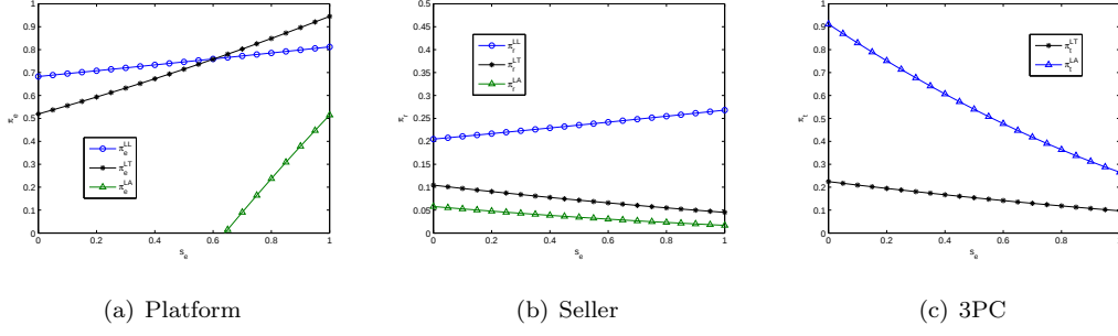
FIGURE 2. Effects of s_e on the profits of supply chain members in modes LL, LT, and LA ( s_t = 0.1 , c_e = 0.1 , c_t = 0.1 , f = 0.5 )
