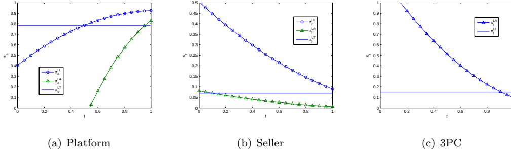
FIGURE 6. Effects of f on the profits of supply chain members in modes LL, LT, and LA ( s_e = 0.8 , s_t = 0.3 , c_e = 0.1 , c_t = 0.1 )
