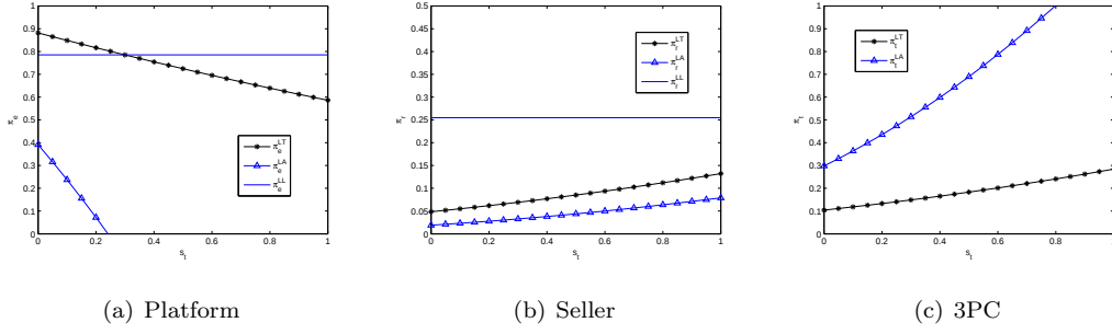
FIGURE 3. Effects of s_t on the profits of supply chain members in modes LL, LT, and LA ( s_e = 0.8 , c_e = 0.1 , c_t = 0.1 , f = 0.5 )
