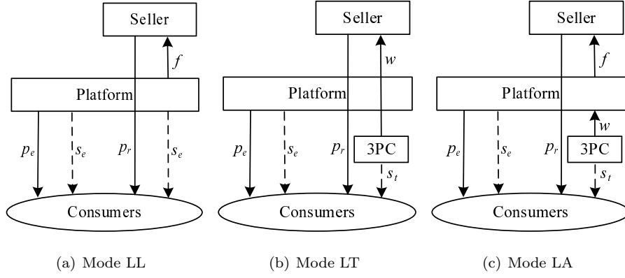
FIGURE 1. Mode structures for the online supply chain
