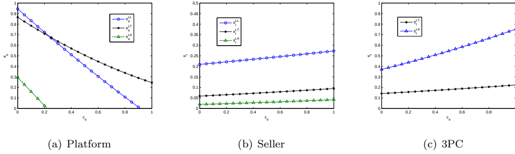
FIGURE 4. Effects of c_e on the profits of supply chain members in modes LL, LT, and LA ( s_e = 0.8 , s_t = 0.3 , c_t = 0.1 , f = 0.6 )
