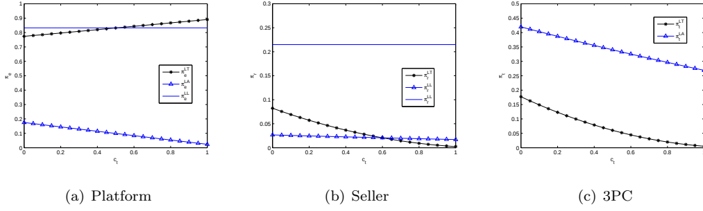
FIGURE 5. Effects of c_t on the profits of supply chain members in modes LL, LT, and LA ( s_e = 0.8 , s_t = 0.3 , c_e = 0.1 , f = 0.6 )
